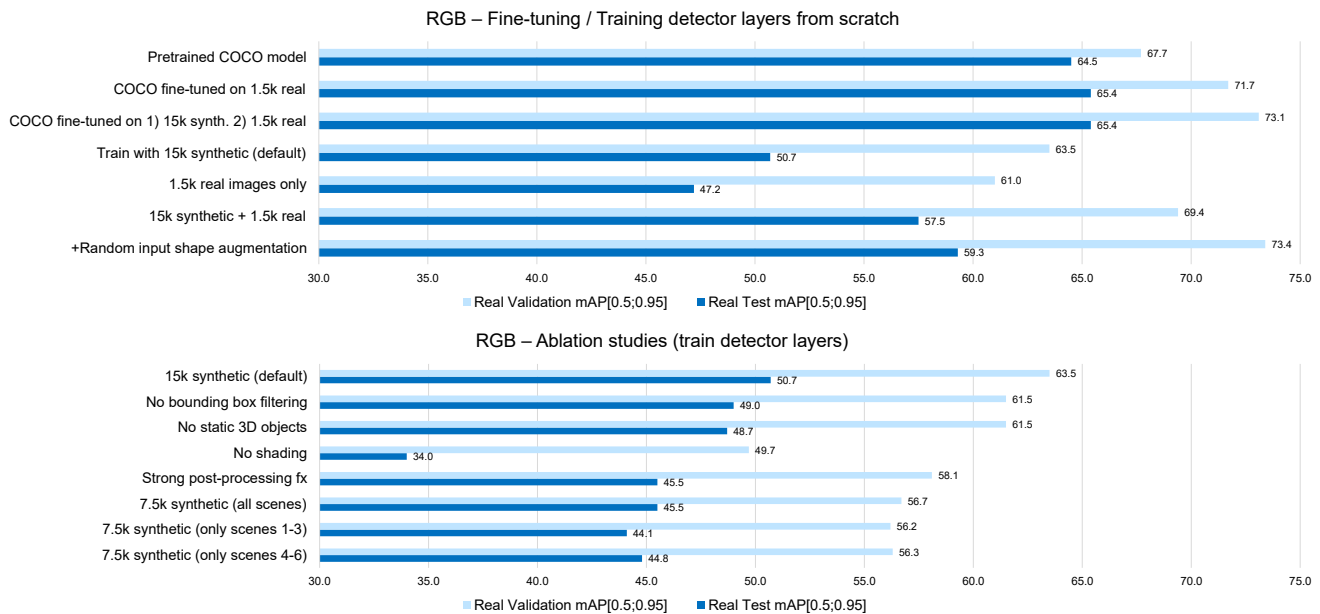
Figure 7: Synthetic RGB training results. Validation and testing on real-world intralogistics dataset.
