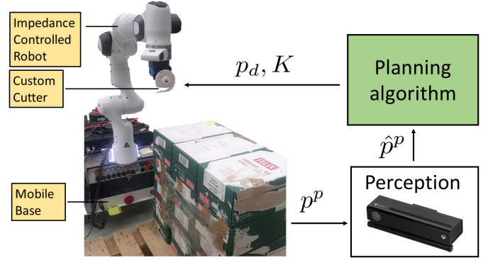
Fig. 1. Architecture of the envisioned system: the perception system acquires information of the pallet ( p^p ) and provides an estimate to the planning algorithm ( \hat{p}^p ), which computes reference trajectory and Cartesian impedance ( p_d, K ) for the impedance-controlled robot mounted on a mobile base and equipped with the custom cutting end-effector.
